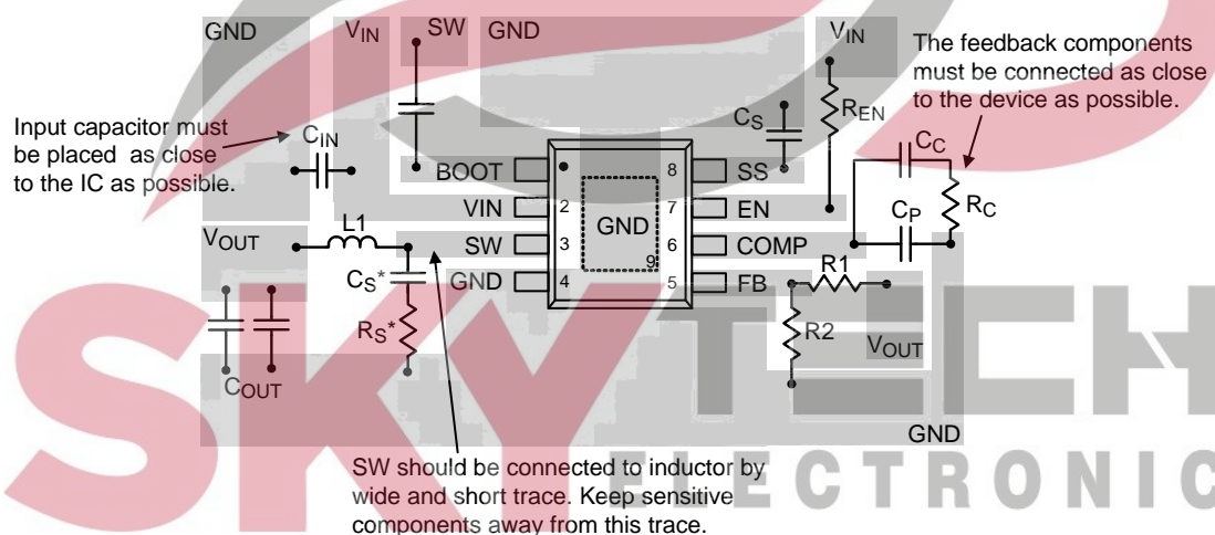
Figure 8. PCB Layout Guide
